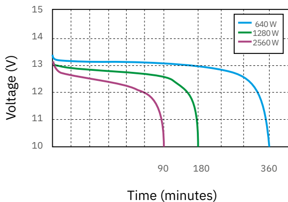
Constant Power Discharge Characteristics (25°C Ambient Temperature)
